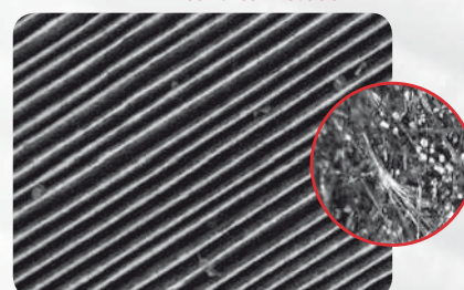
Filter after 15.000 km
